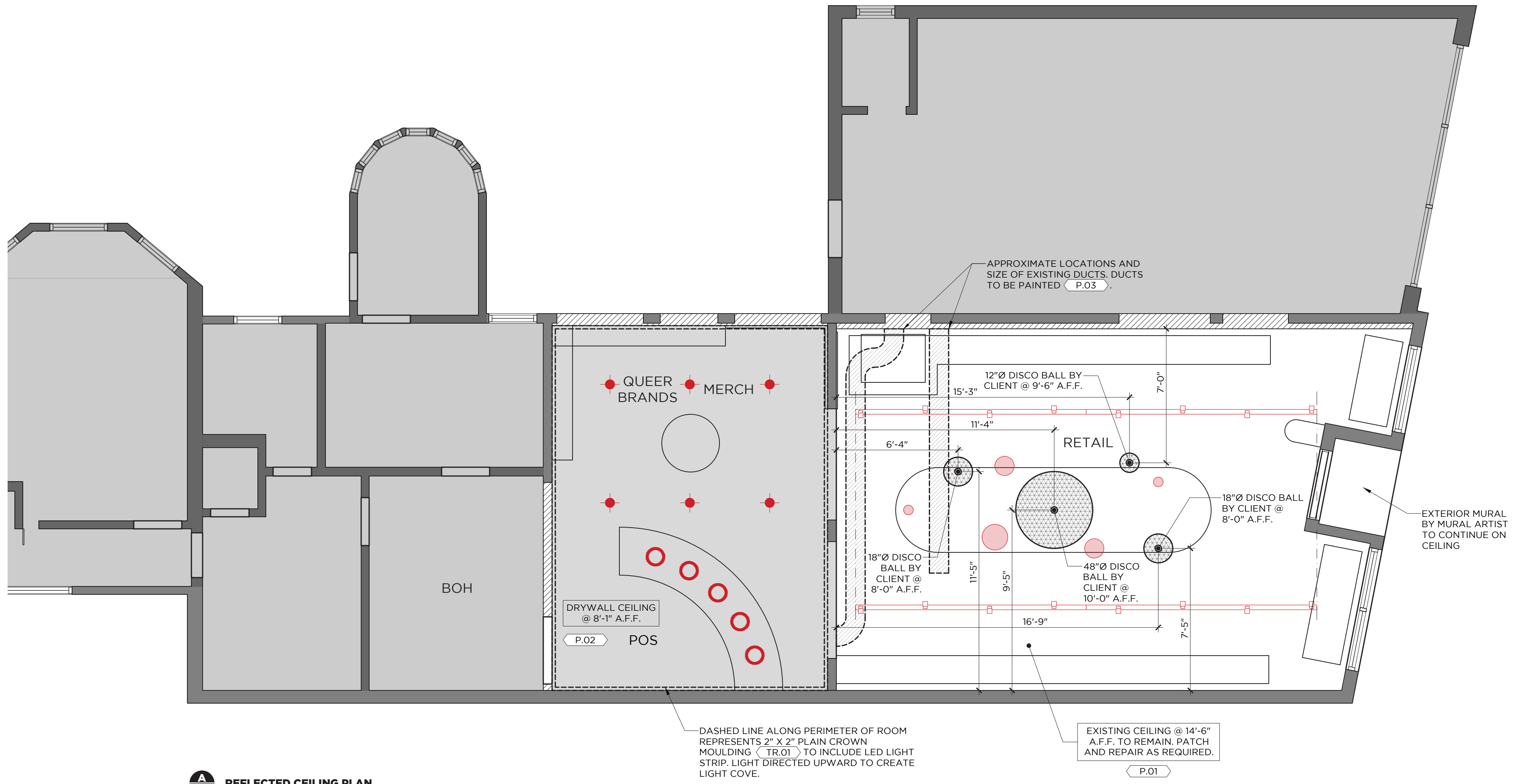
A REFLECTED CEILING PLAN
