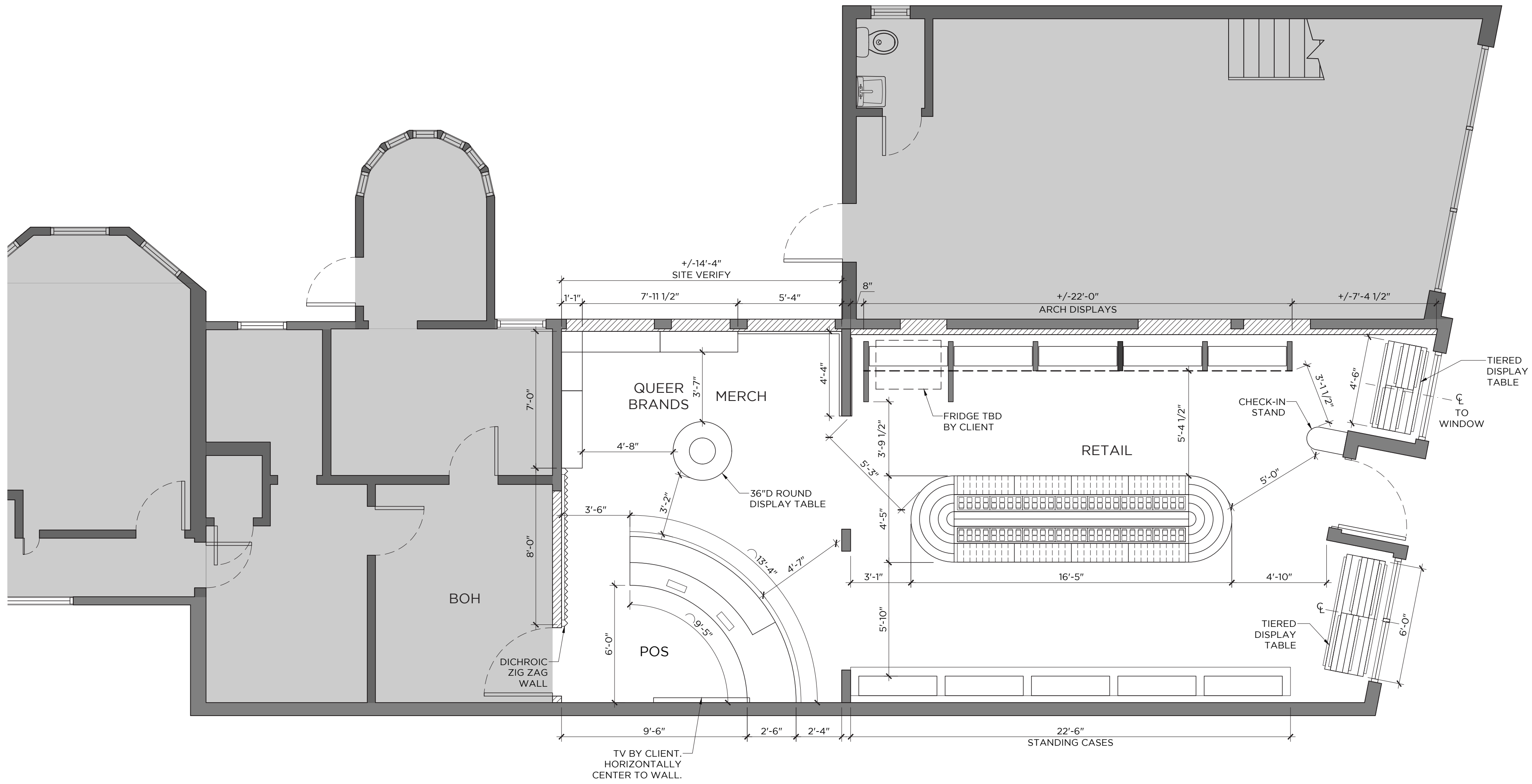
A 6 FIXTURE PLAN
