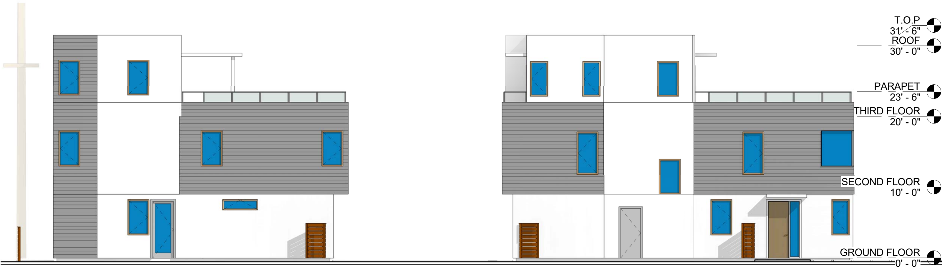
1 NORTH ELEVATION 1/8" = 1'-0"
